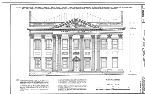
Measured drawing of the First Bank from the Historic American Buildings Survey. [24]
