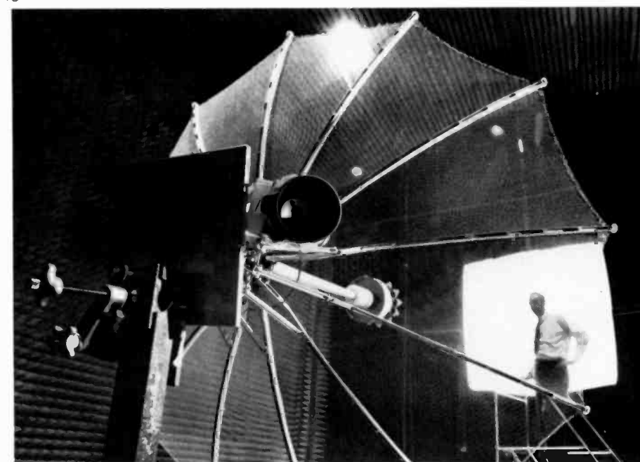
16. An engineer at RCA's Missile and Surface Radar Division, Moorestown, N.J., supervises space chamber tests of a folding antenna of the kind that will transmit color TV and other communications from Apollo 15 astronauts' Lunar Rover "space taxi" as it roams the moon. The antenna, with spined sections of gold mesh, opens and closes like an umbrella.
