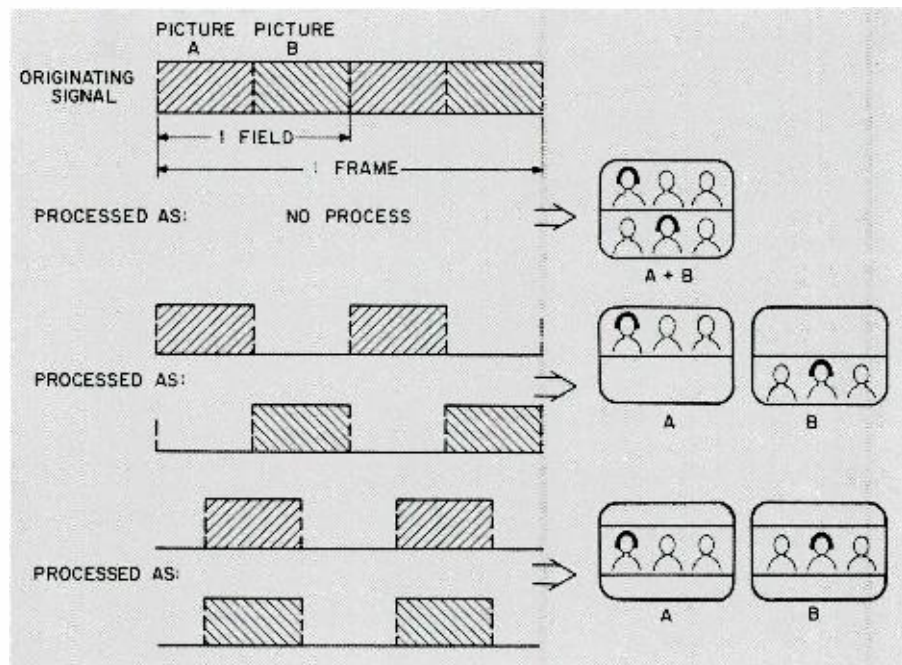
Fig. 7. Scene separation techniques.
