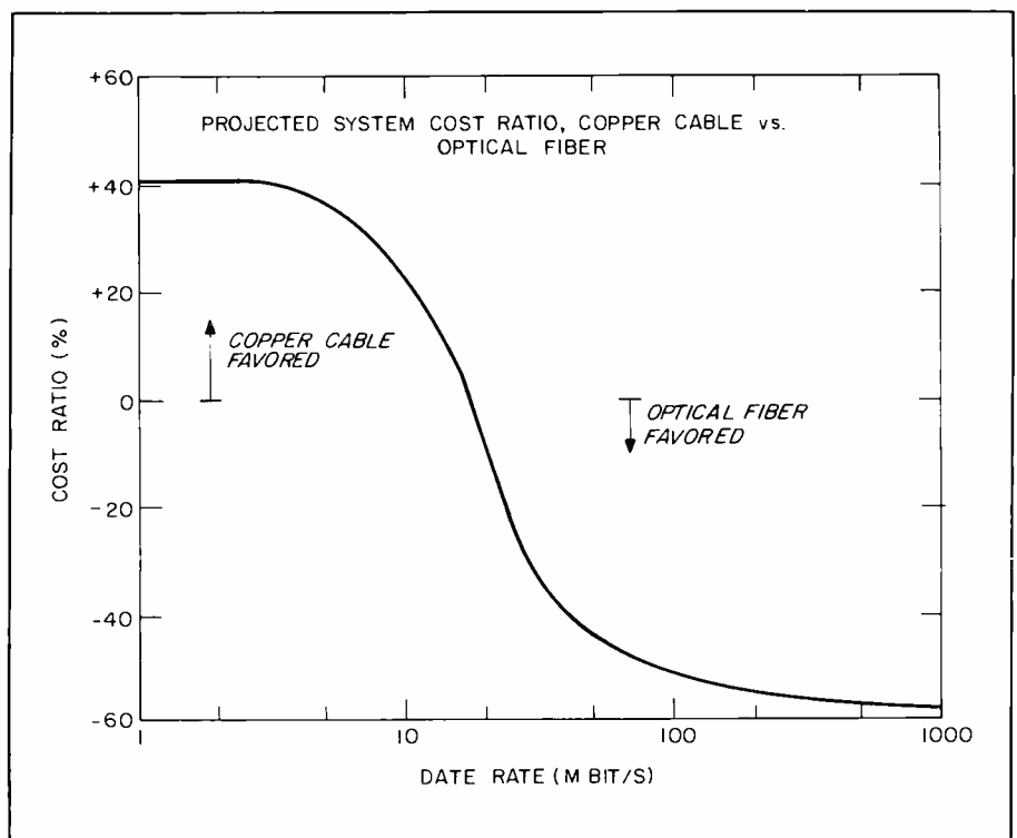
Fig. 25. Cost comparison of copper cable and optical fiber systems versus data rate.
