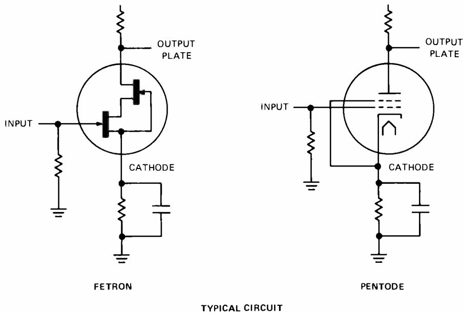
Fig. 5. The Junction Field Effect Transistor (left) illustrates one approach to the gradual yet efficient application of higher technology in older (right) systems. Economics dictate that state-of-the-art designs maintain technical and operational compatibility with the telephone network.
