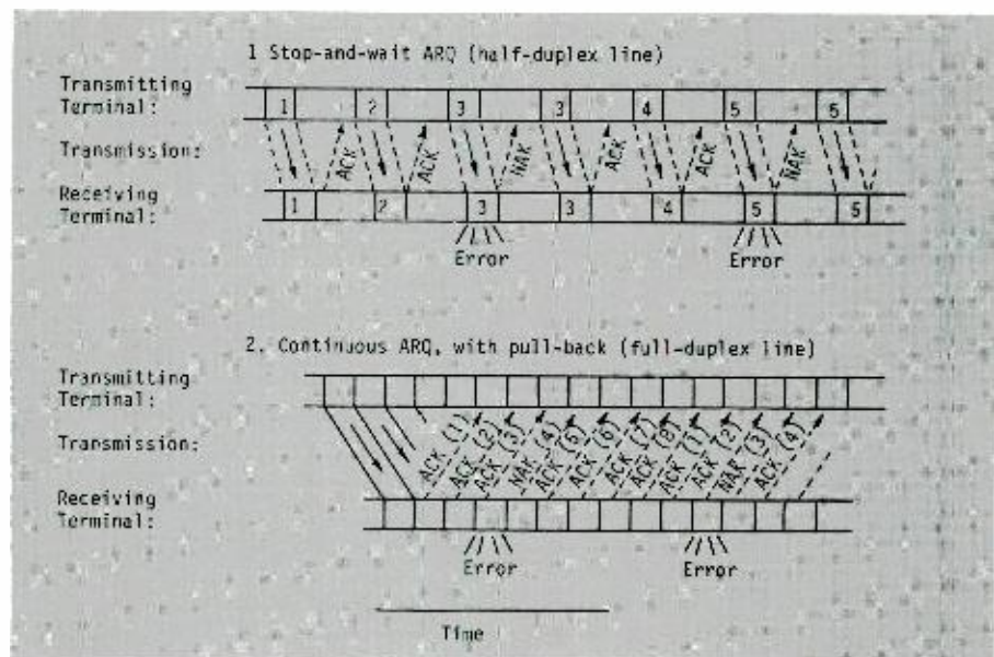
Fig. 1. With stop-and-wait ARQ, much time is spent waiting for acknowledgment. Continuous ARQ rectifies this by permitting blocks to be sent before previous blocks are acknowledged.
