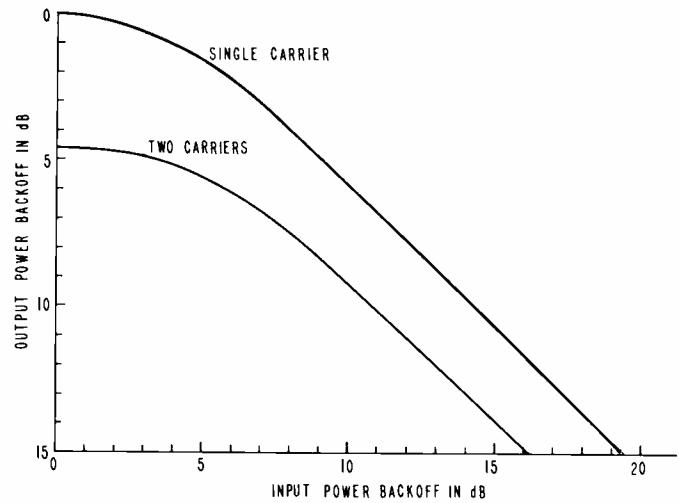
Fig. 6. TWTA output power versus input power characteristic.
