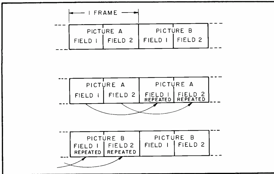
Fig. 8. Alternate frame multiplexing and frame repeat demultiplexing.
