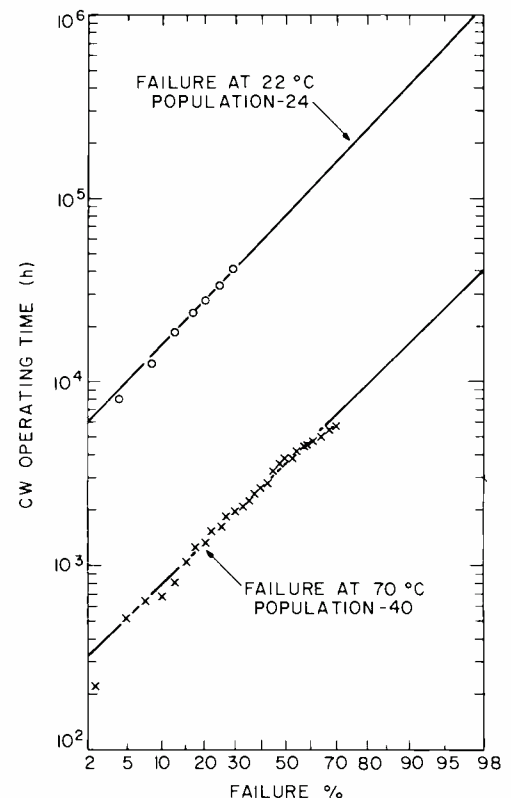
Fig. 14. Log-normal plot of mean time to failure for AlGaAs lasers at 22^\circ and 70^\circ C .
