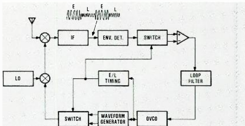
Fig. 11. Early/late range tracker. This phase-locked loop uses the E-L error signal from Fig. 10 to force the nominal system timing, which is exactly halfway between the early and late waveforms generated locally, to equal the received waveform timing. The early and late waveforms are alternately selected for short periods and the error signal is integrated over many periods in the loop filter.
