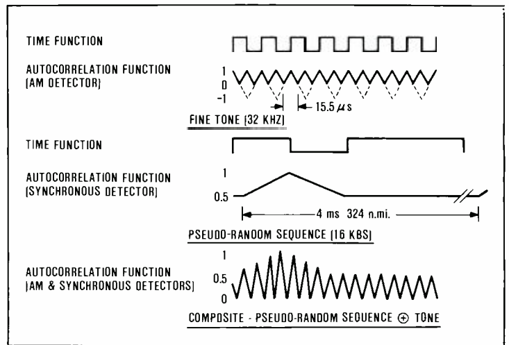
Fig. 8. Correlation of PSK/AM ranging waveform. The correlation function measures the degree of agreement between two waveforms as the waveforms are time-shifted through their full period. The correlation functions of the fine-tone and the pseudo-random code are multiplied together to provide the composite correlation function. The highest peak is accurately tracked to measure the ranging waveform.
