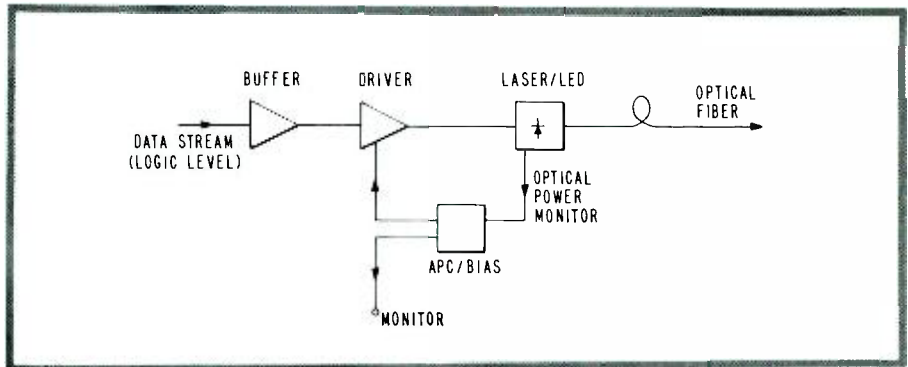
Fig. 16. Components of a fiber optic transmitting system.
