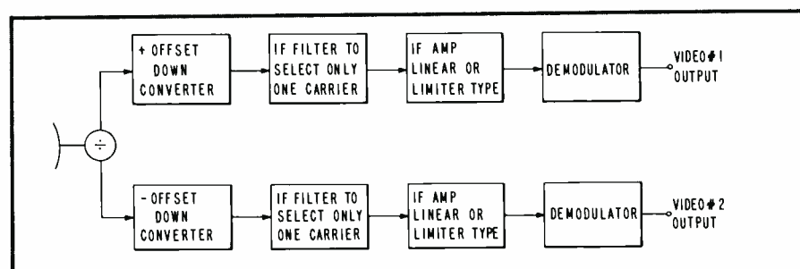
Fig. 10. Implementation of two-carrier system at receiver site.
