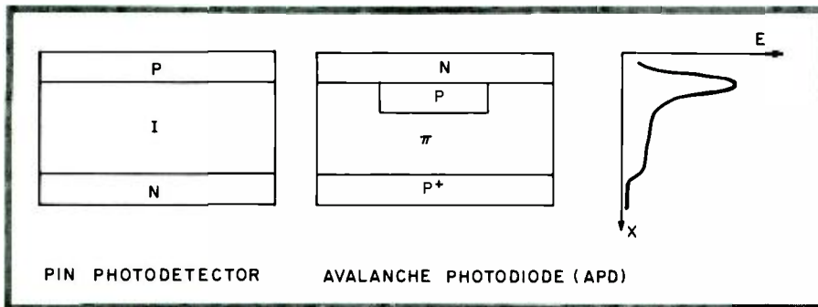
Fig. 12. Sketch of PIN detector and an avalanche photodiode.
