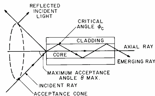
Fig. 1. Ray diagram that shows the maximum angle of incidence for light to be accepted by and propagated in an optical fiber.
