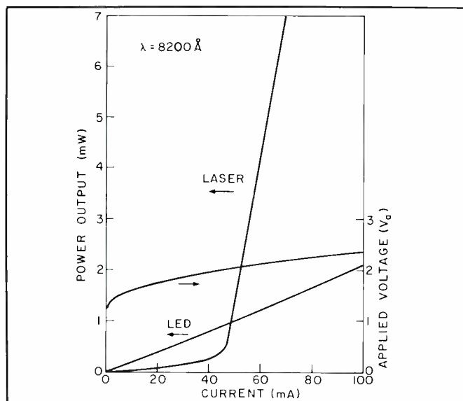
Fig. 7. Output power versus input current for lasers and LEDs.
