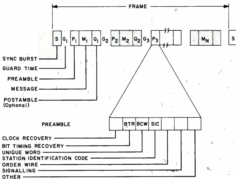
Fig. 4. Overhead in a time-division multiple-access (TDMA) system consists of bits used to label and control the blocks, as well as guard time between them.
