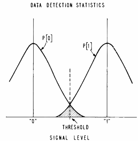
Fig. 22. Overlap between a "zero" and a "one" pulse—both of which are distributions.
