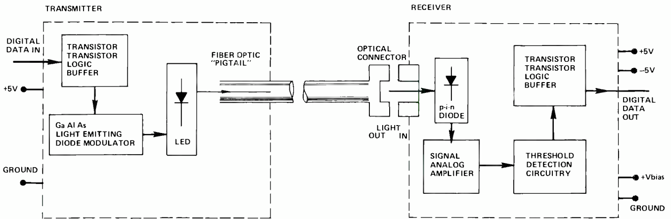
Fig. 10. Circuitry for device electronics used for RCA lasers and LEDs.
