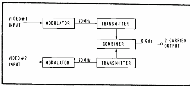
Fig. 5. Implementation of two-carrier system at transmitter site.
