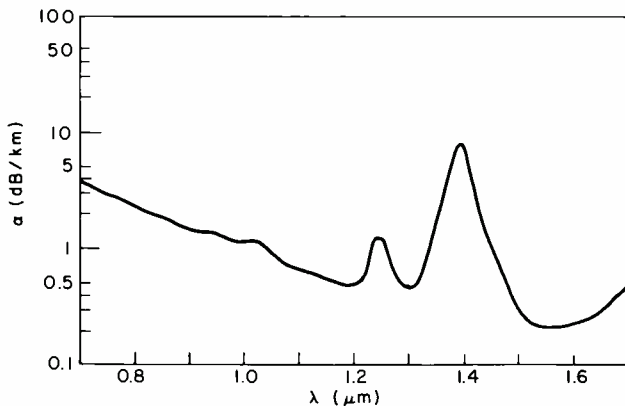
Fig. 3. Attenuation loss versus wavelength for high-quality silica fibers.
