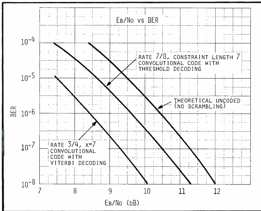
Fig. 3. Various types of forward-error-correction coding provide different levels of performance.
