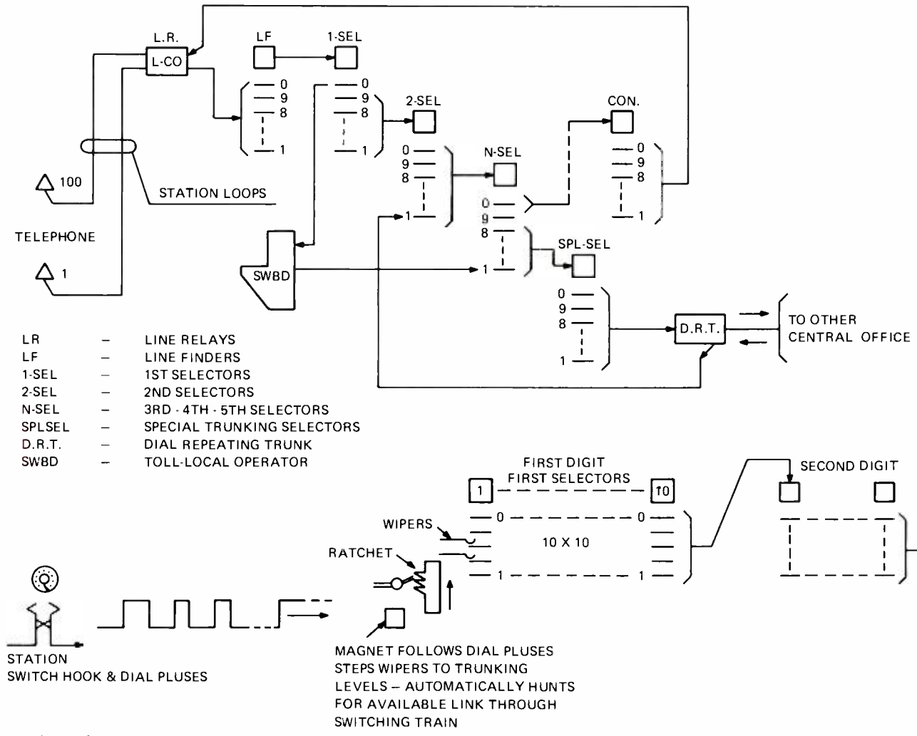
Fig. 4. Direct Control systems consist of many individual switches. The switching mechanisms of each unit are under direct control of the calling party's dial pulses. The call is processed in a pseudo-random pattern through groups of switches representing each digit.
