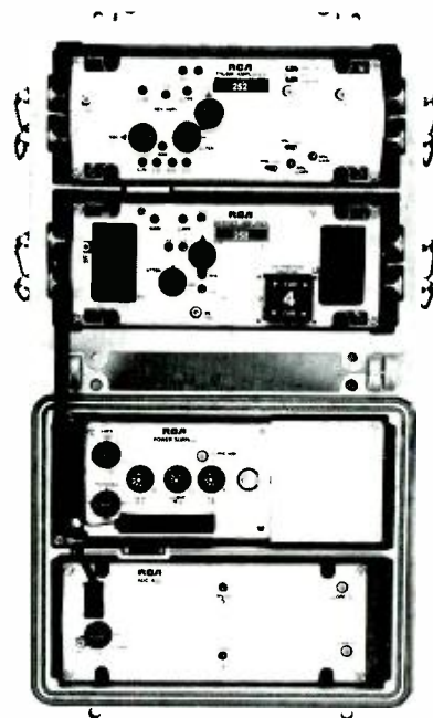
Fig. 3. Trunk bridger amplifier with cover open.
