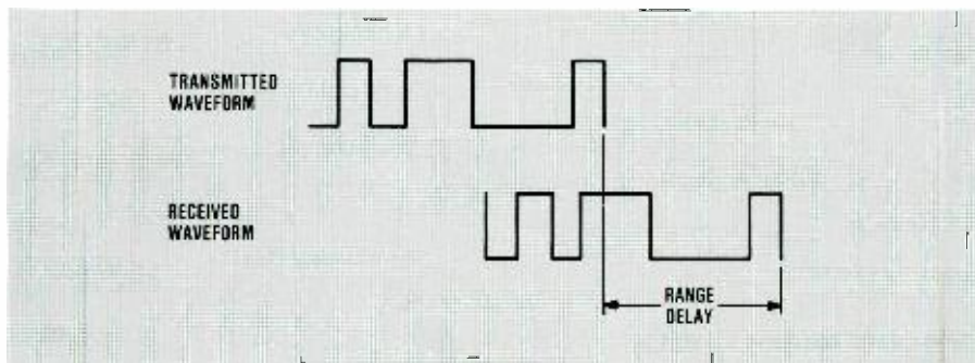
Fig. 2. Range measurement with pseudo-random code. The range is directly proportional to the phase shift or delay between the transmitted and received waveforms, whether that waveform is a tone or a pseudo-random code.
