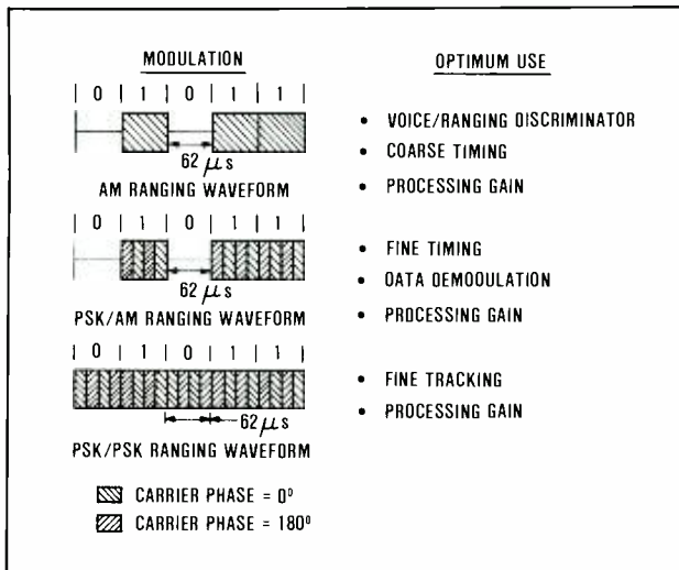
Fig. 7. Ranging modulations. Different combinations of AM and PSK modulation are used with the fine-tone and pseudo-random code to provide solutions to different system requirements.
