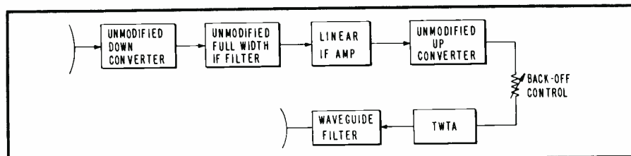
Fig. 9. Single channel two-carrier repeater configuration.
