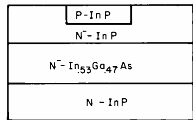
Fig. 13. Novel structure of a long ( > 1 \mu m ) wavelength photodetector. Light absorption takes place in the low-bandgap InGaAs layer, whereas current is collected across the P/N junction in the high-bandgap InP .
