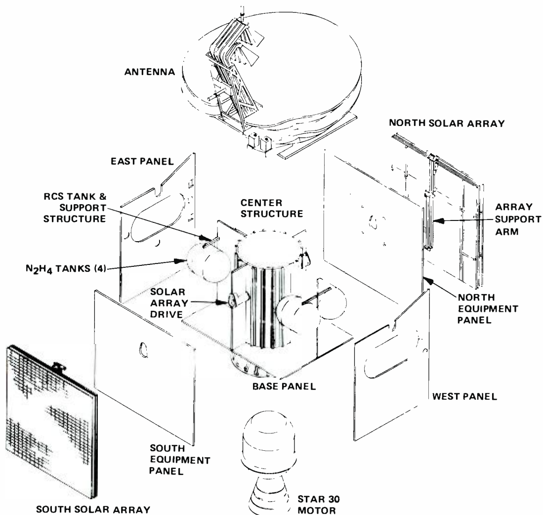
Fig. 6. Spacecraft structure. Lightweight modular structure retains proven features of Satcom while accommodating more equipment weight and power.
