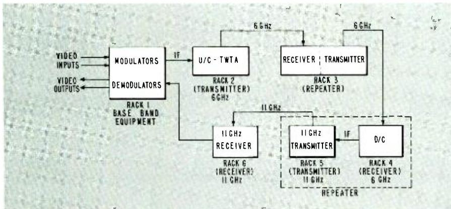
Fig. 3. Experimental three-hop microwave radio system.
