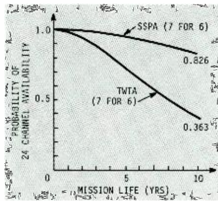
Fig. 5. Power amplifier availability comparison. Lower parts-count and absence of filament-heated cathode contribute to higher reliability of SSPA compared to TWTA.
