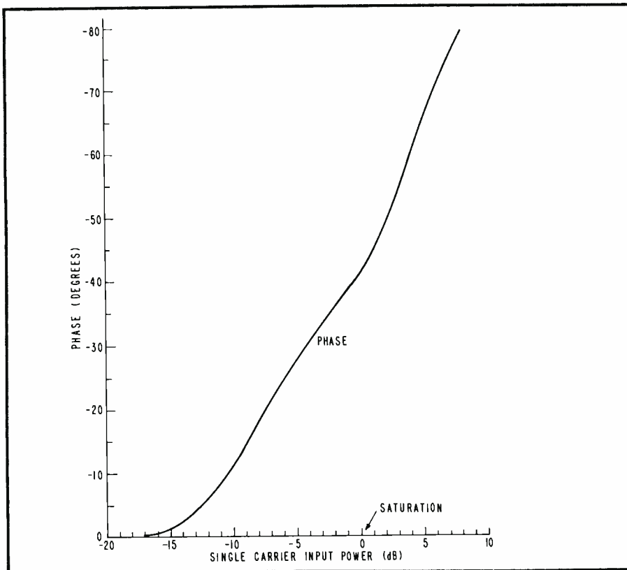
Fig. 7. TWTA output phase versus input power characteristic.
