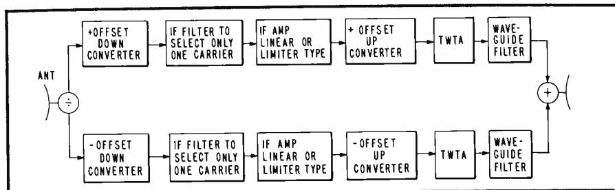
Fig. 8. Dual channel two-carrier repeater configuration.
