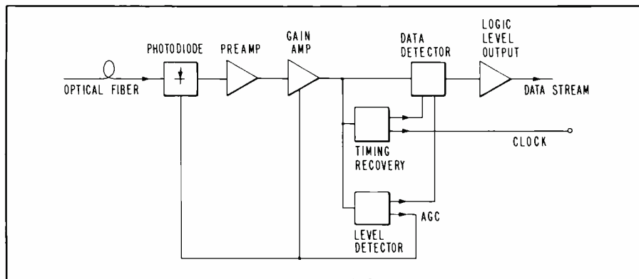
Fig. 18. Basic layout for an optical data receiver.
