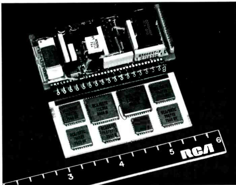
Fig. 14. Engineering model of the transponder. The complete module occupies two cubic inches when folded in half for insertion into the handheld radio.
