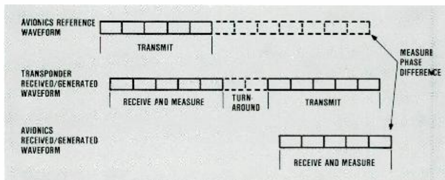
Fig. 3. Half-duplex ranging system timing. In the half-duplex ranging system, the radios cannot transmit and receive at the same time. Therefore, the ranging waveform frequency and phase must be precisely measured and controlled at the transponder for accurate replication during the transponder transmit period.
