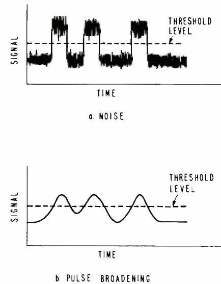
Fig. 21. Pulse degradation due to (a) noise and (b) pulse broadening.
