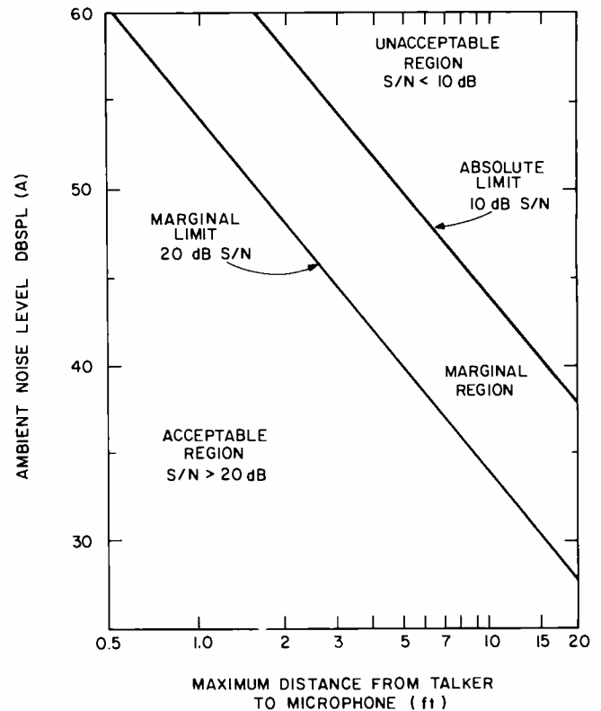
Fig. 2. Microphone/talker separation.
