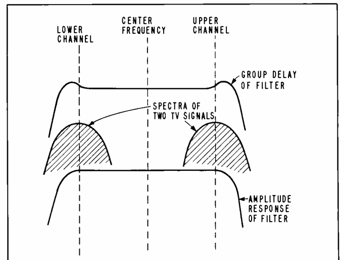
Fig. 16. FM to AM conversion mechanism for carriers with excessive spacing.
