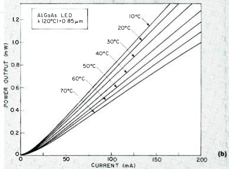
Fig. 11. Output power versus input current as a function of temperature for (a) lasers and (b) LEDs.
