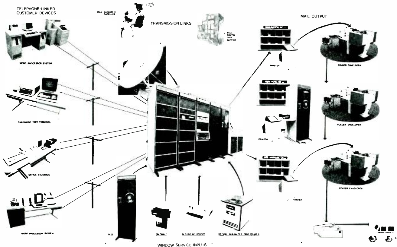
The Evaluation and Test System (ETS), developed and shipped in a 12-month span, was based mostly on existing equipments, but high-resolution facsimile, and low-resolution facsimile interfaces to telephone lines were specially developed. Other input devices were word processors, tape cartridge readers, tape readers and optical character readers (OCR). Output letters are computer-formed to include stored logos, signatures and business forms. Approximately 100,000 in-core instructions were specially developed for the system.
