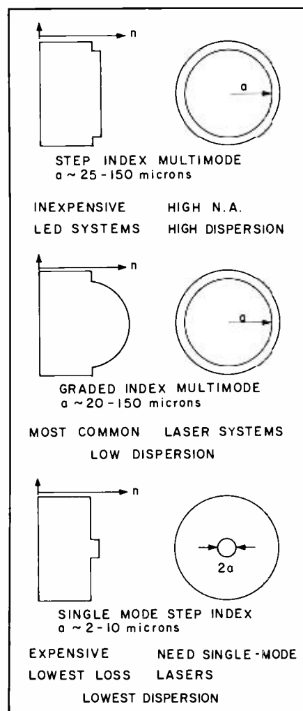
Fig. 2. Three main types of optical fibers.
