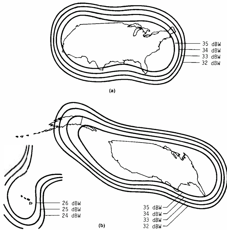
Fig. 3. Advanced Satcom EIRP coverage. (a) Eastern orbital positions. (b) Western orbital positions. Antenna "footprints" are matched to the service area for maximum efficiency.
