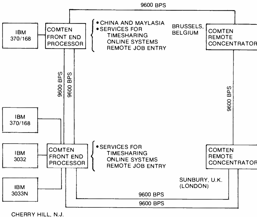
Fig. 5. Geographically dispersed customers can gain access to the IDN through the COMTEN nodes. In the event of line failure, alternate paths are automatically selected.
