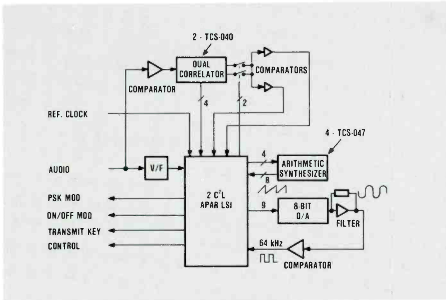
Fig. 13. Transponder block diagram. An extremely high level of integration is achieved with four digital LSI circuit types. The A/D, D/A and few analog functions required four dual inline packaged ICs.
