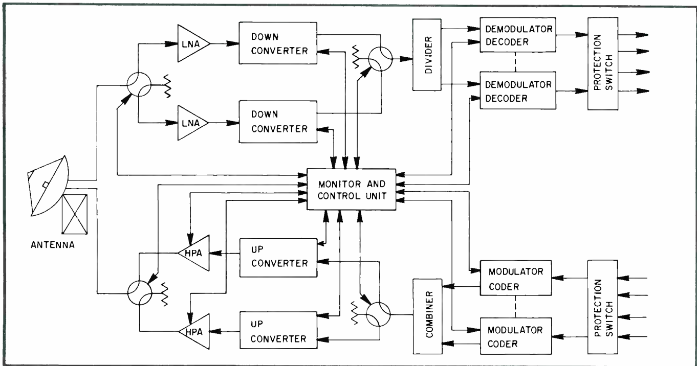
Fig. 2. The redundancy of all critical elements and continuous alarm monitoring are shown in this block diagram of a typical 56-Plus earth station.
