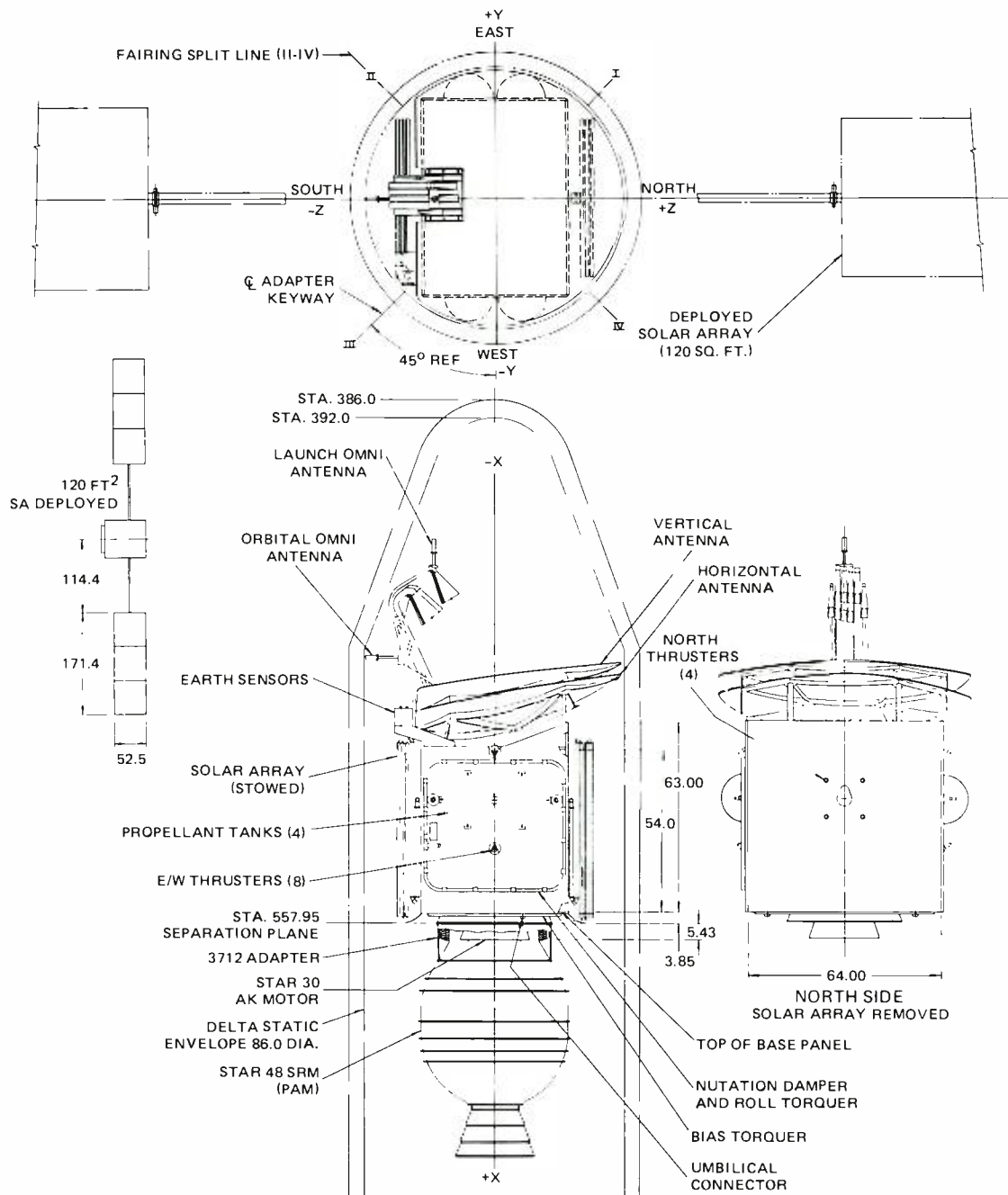
Fig. 7. Delta launch configuration. Spacecraft with new antenna maintained compatibility with the volume limits of the Delta launch vehicle.
