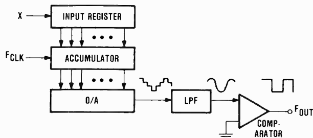
Fig. 12. Basic digital VCO (arithmetic synthesizer). A number X is added into the accumulator on each clock pulse. The DVCO output frequency is the rate of overflow of the accumulator. The cleanup circuits on the output signal reduce the jitter introduced by the time quantization.
