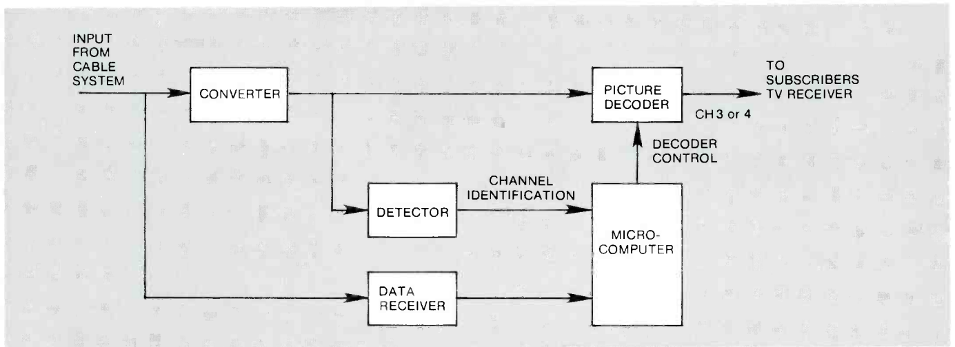
Fig. 5. Subscriber terminal.
