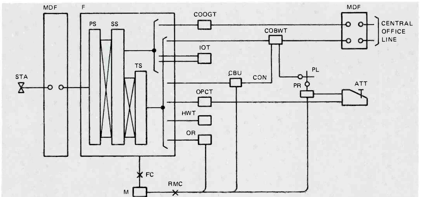
TYPICAL TRUNKING DIAGRAM FOR COMMERCIAL SYSTEM
