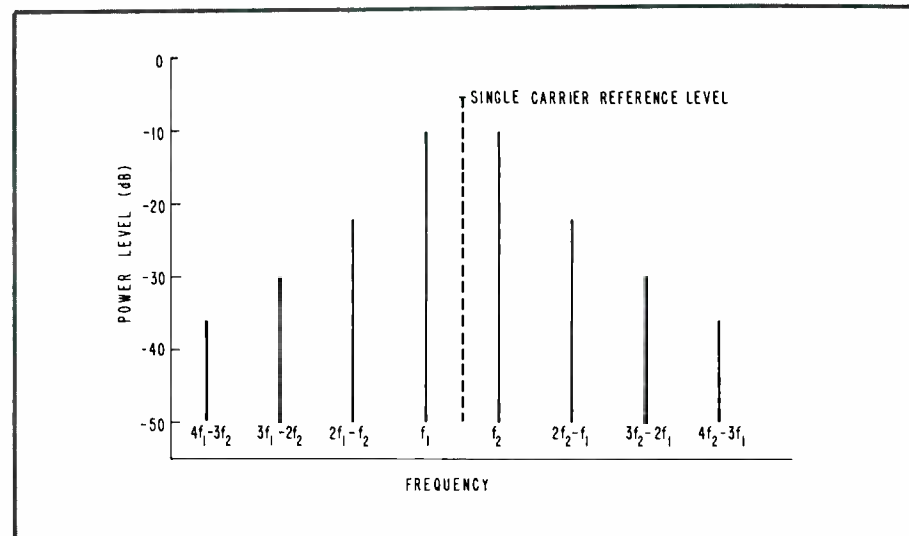
Fig. 12. Two-tone intermodulation spectrum of TWTA operating at saturation.
