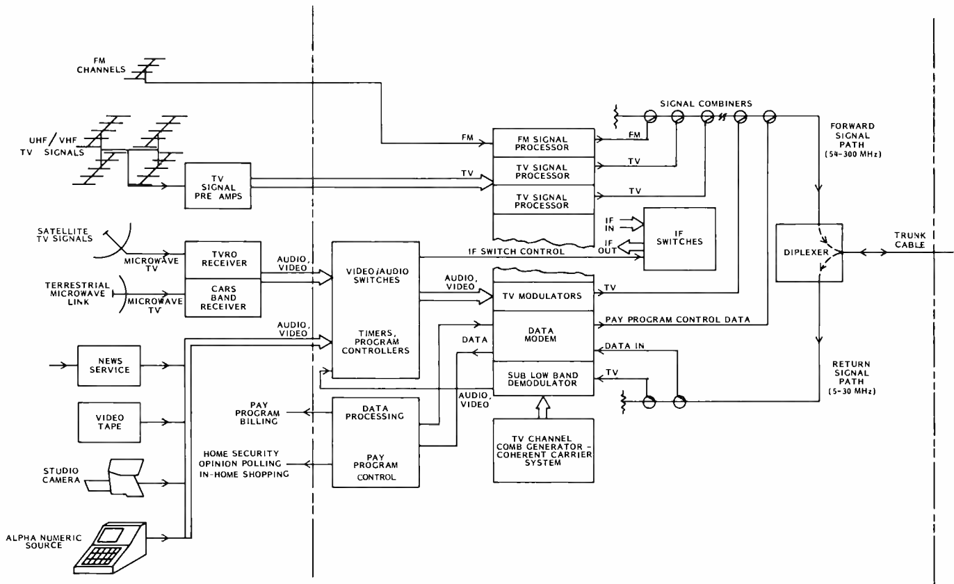
Fig. 1. Typical full-service CATV headend.
