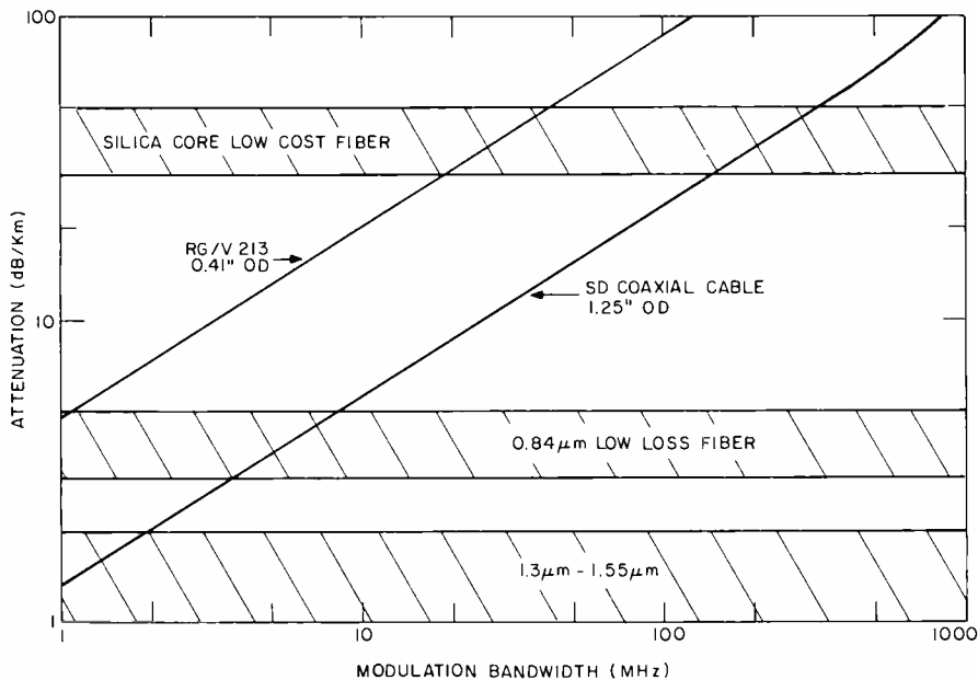
Fig. 17. Attenuation loss versus modulation bandwidth for coaxial cable and optical fibers.
