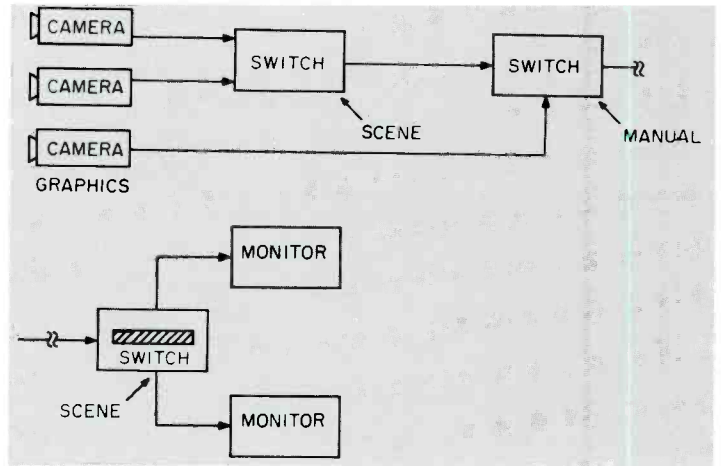
Fig. 9b. Optional scene separation at receiver.
