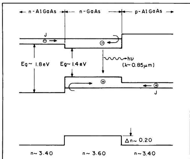
Fig. 6. Energy-bandgap step and refractive-index step for GaAs/-AlGaAs double-heterostructure laser.
