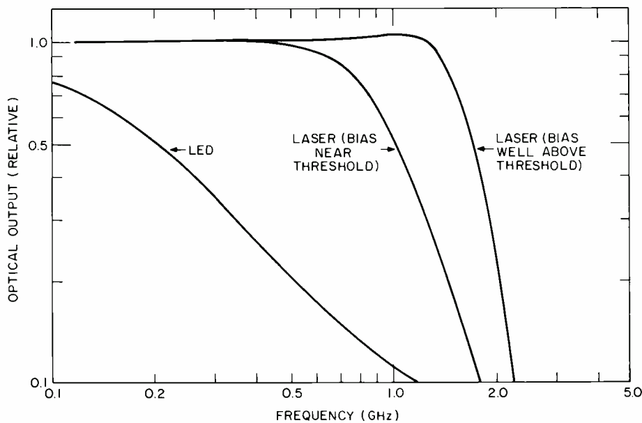
Fig. 8. Relative output versus frequency for LEDs and lasers.
