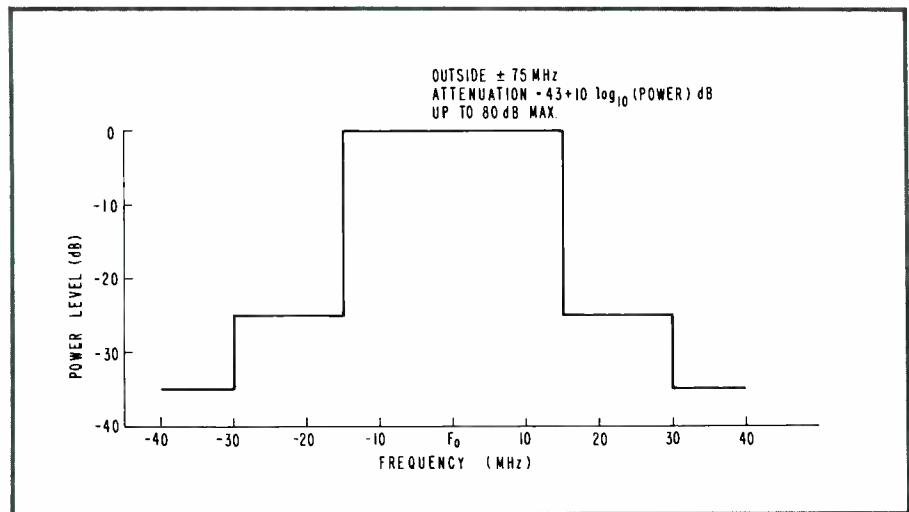
Fig. 11. FCC mask for spurious response in the 6-GHz band.
