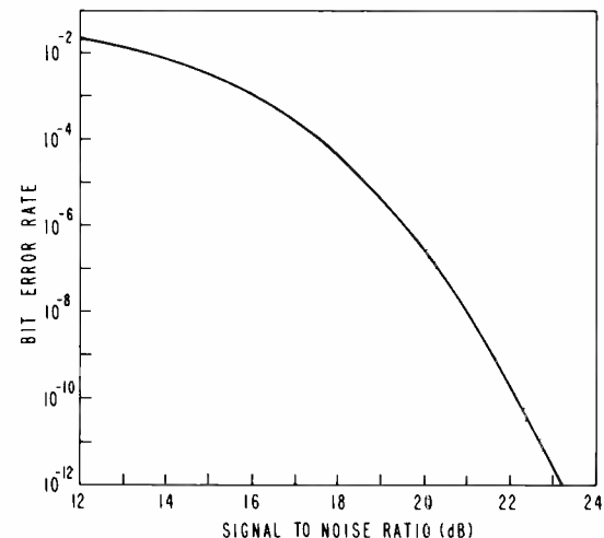
Fig. 23. Bit-error rate (BER) versus signal-to-noise ratio for a fiber optical system.
