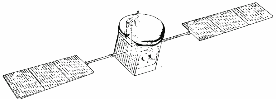
Fig. 2. Advanced Satcom on-orbit configuration. Second-generation Satcom features new antenna design and larger solar array for more traffic capacity.
