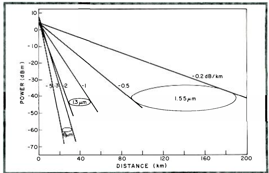
Fig. 4. Total loss (in dBm: referenced to 1mW) versus distance in fiber optical systems operating at 0.85 \mu\text{m} , 1.3 \mu\text{m} and 1.55 \mu\text{m} .
