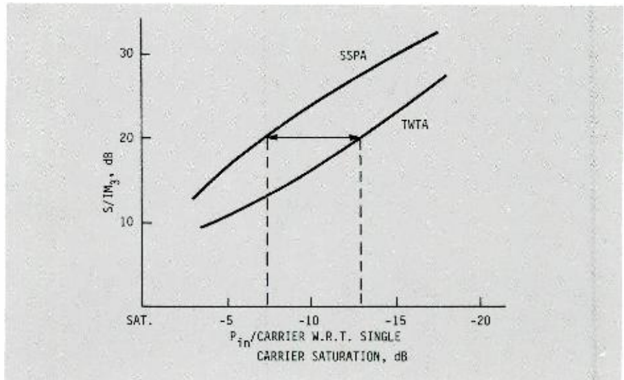
Fig. 4. Amplifier linearity comparison. SSPA linearity results in lower intermodulation distortion than available with TWTA.
