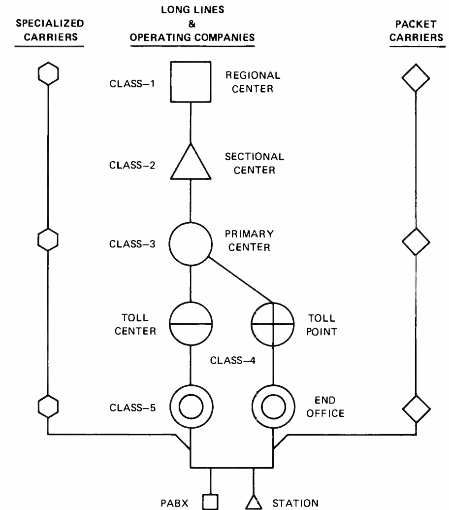
Fig. 2. The telephone network hierarchy is compared with tandem switching or processing modes of the newer competitive voice and data carriers.
