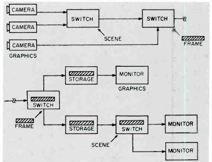
Fig. 9d. A complete system.
