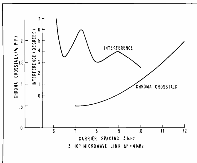
Fig. 15. Crosstalk versus carrier spacing.
