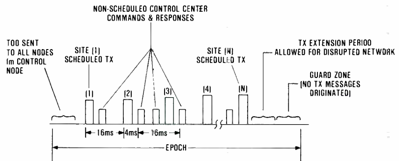
Fig. 2. Network timing.
