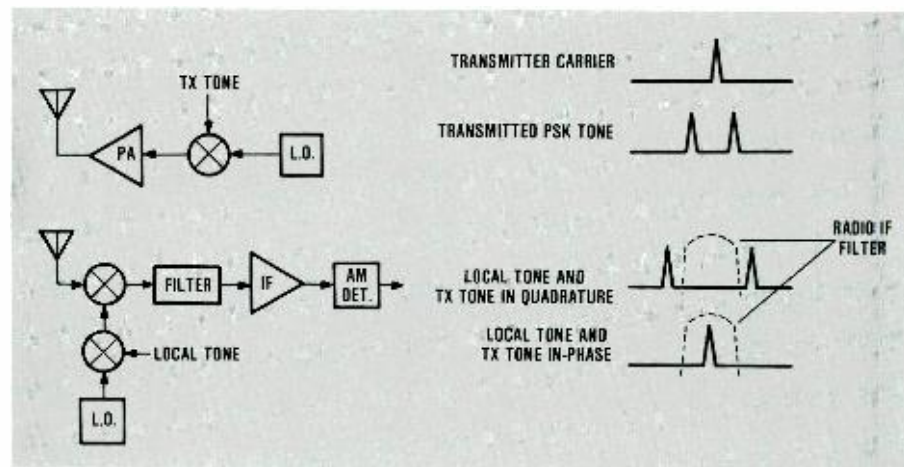
Fig. 6. Spectrum correlation. The reciprocal properties of bi-phase PSK modulation are used to provide a correlation function of the ranging waveform. As the phase relationship of TX tone and local tone shifts from quadrature to in-phase, the signal energy in the IF increases linearly.
