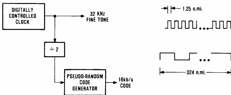
Fig. 5. Ranging waveform generator and waveforms. The ranging waveform combines a fine tone with a pseudo-random code. The fine tone provides accuracy by supplying many transitions for edge tracking. The pseudo-random code provides the equivalent of a coarse tone to resolve range ambiguities out to 324 nautical miles.
