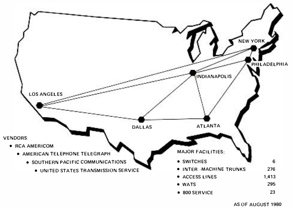
Fig. 1. Electronic switchers located in the cities shown are interconnected to form the backbone of the TACNET network.
