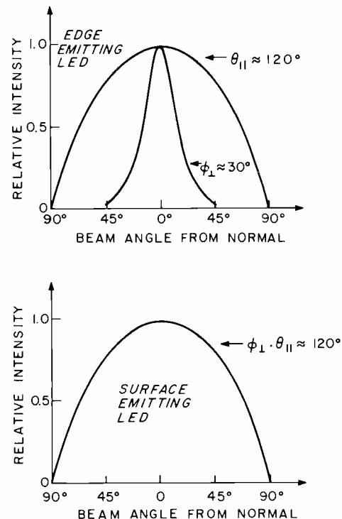
Fig. 9. Far-field beam patterns for edge-emitting and surface-emitting LEDs.
