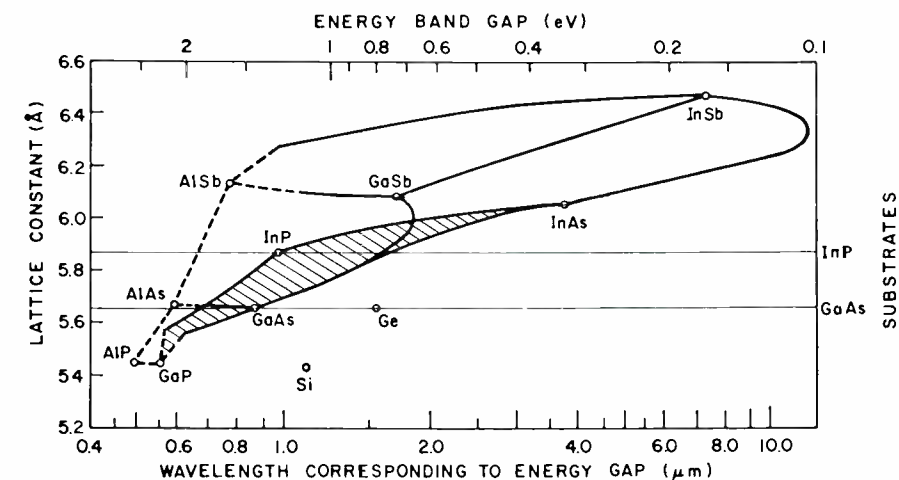
Fig. 5. Energy bandgap and lattice parameter for binary, ternary and quaternary III - V compounds.
