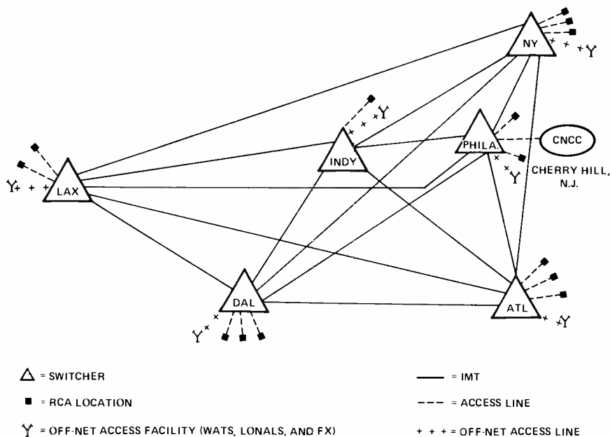
Fig. 2. The interrelationships of the major TACNET components are graphically depicted above.
