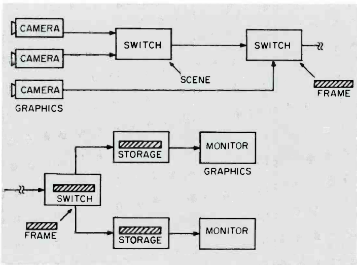
Fig. 9c. Scene interleaving and frame multiplexing.
