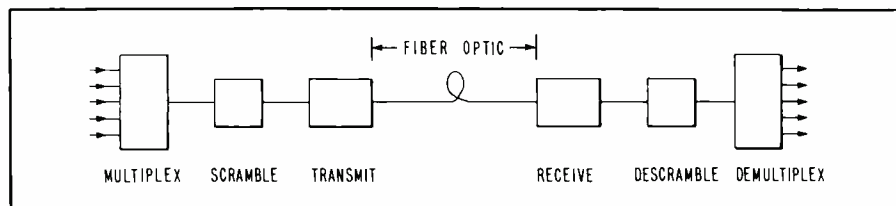
Fig. 19. Complete optical data link.
