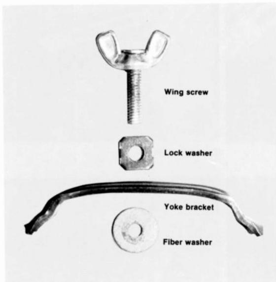
Fig. 1 Is automatic assembly possible? Engineers must examine each group of parts to determine the best method of assembly—hand, semiautomatic, or automatic. This group of parts, the yoke wing bracket assembly, is put together by the automatic machinery shown in Fig. 2.
