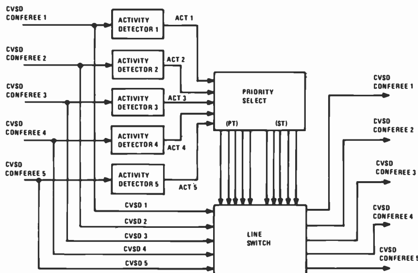
Fig. 8 Activity selection system for CVSD digital conferencing. This system requires that speaker priorities be established.
