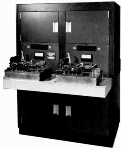
Fig. 3 System II is for production testing. Here, the seven individual test stands have their own controllers and signal sources. Each stand can test two modules independently at the same time. This stand, the signal-package unit, is also shown in block-diagram form in Fig. 4.
