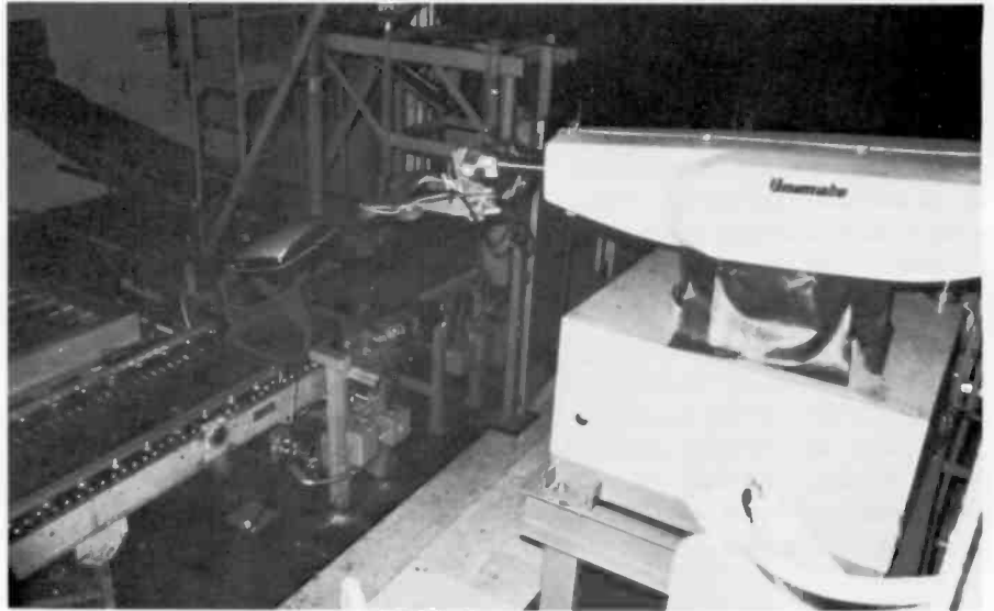
An IR used to unload tubes as they exit from a frit seal lehr and place them on a conveyor hanger for movement to in-line process and test equipment.
